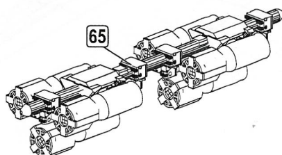
OFAB-100-120 bombs on MBDZ-U6-68 rack
