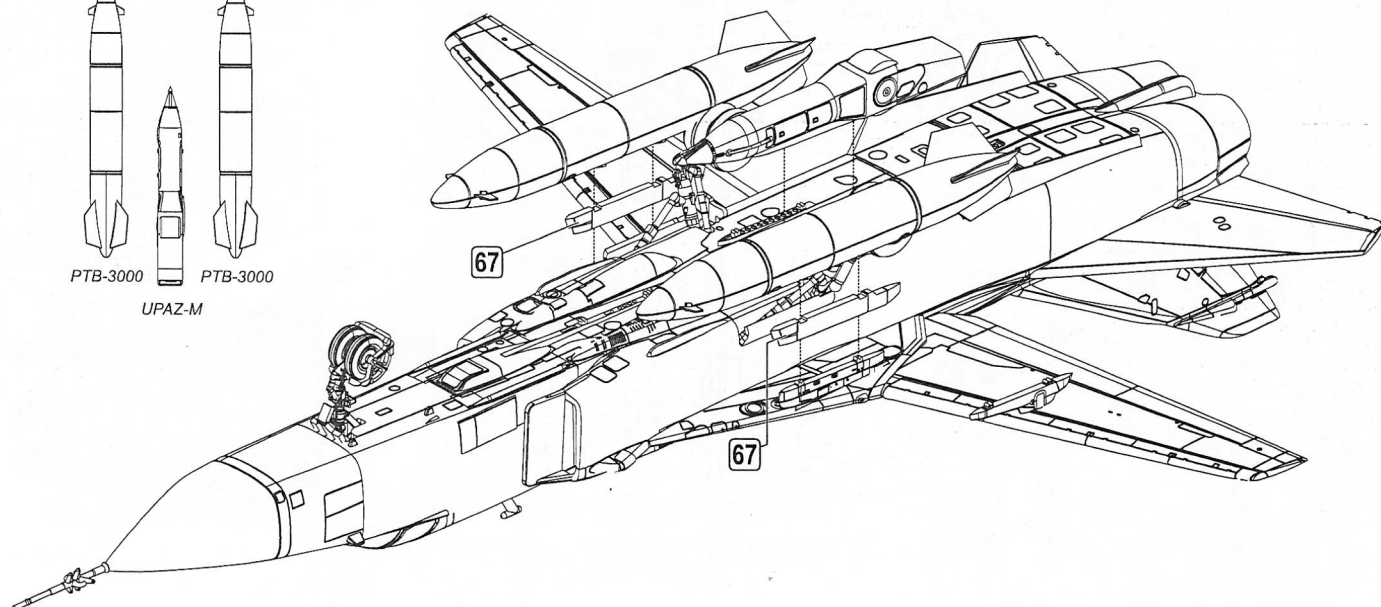
Su-24M aerial refueler version w/ UPAZ-M refueling pod & 2x 3000l fuel drop tanks
