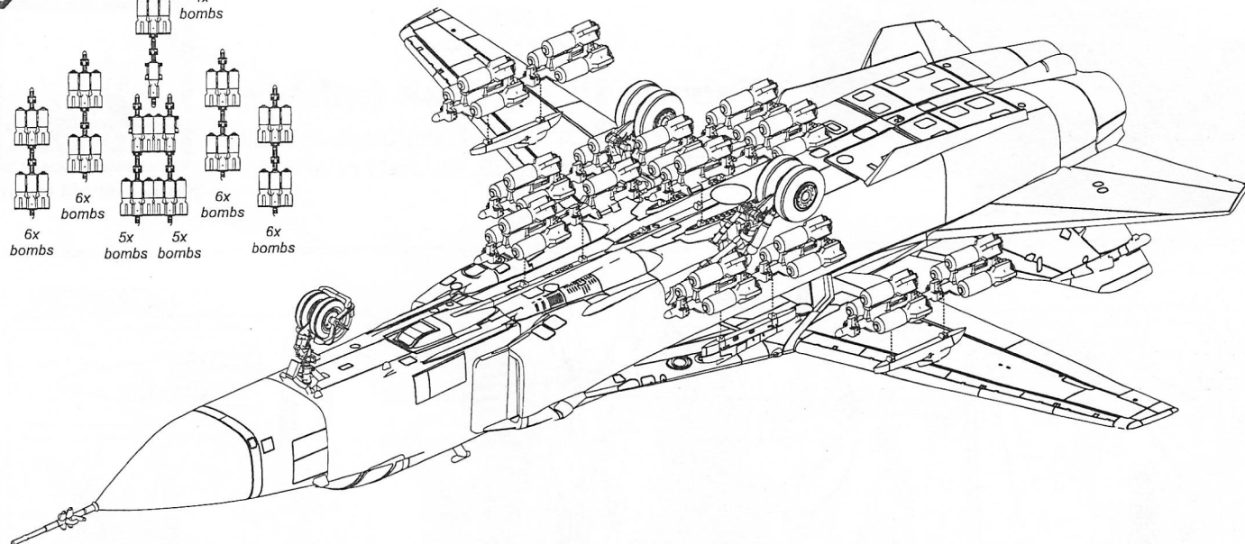
Su-24M bomber version w/ 38x OFAB-100-120 bombs
