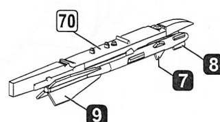
R-60 (AA-8 "Aphid") AA missile on APU-68 launch rail
