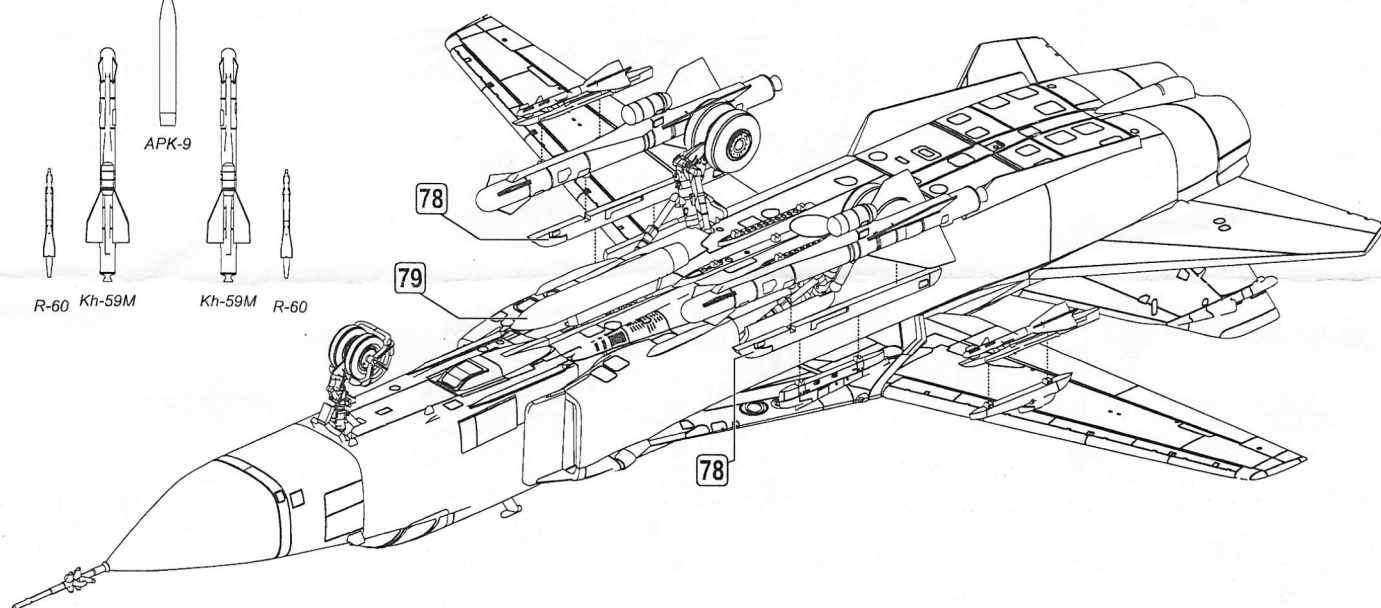
Su-24M missiles carrier w/ 2x Kh-59 "Ovod" cruise missiles
